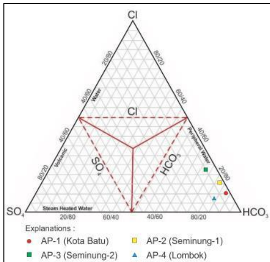
Figure 11: Ternary plot of the major anions Cl - , SO 4 , HCO 3 - for the determination of hot water manifestation type (Hastuti et.al., 2012, Unpublished).
